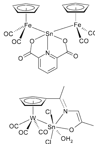
Figure 1. Iron and tungsten half-sandwich complexes with fivefold- and sixfold-coordinated tin atoms.
