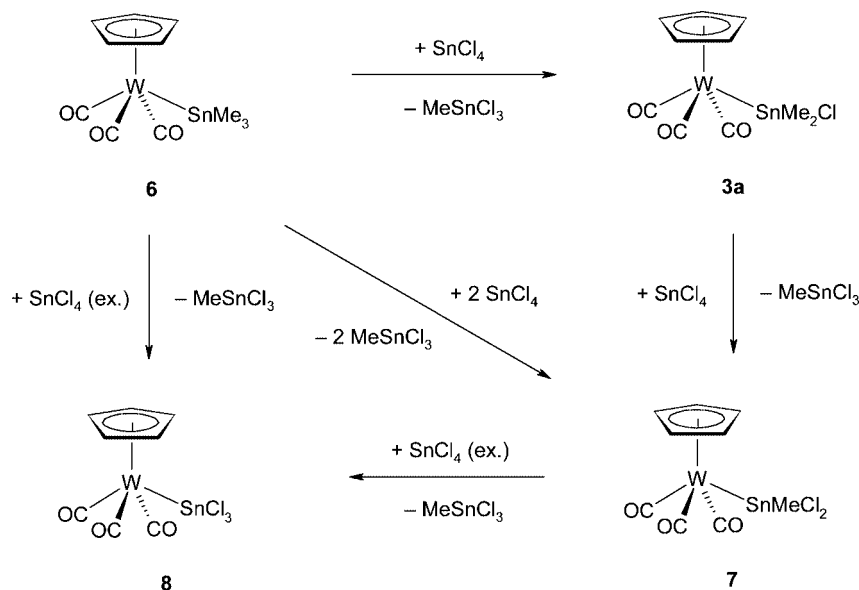
Scheme 2. Stepwise chlorination of 6 via mono- and dichlorinated stannyl tungsten complexes 3a and 7 leading to the trichlorostannyl complex 8 and direct synthesis of 7 and 8 .
