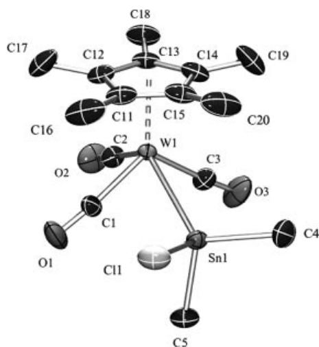
Figure 6. Molecular structure of [(\eta^5\text{-C}_5\text{Me}_5)(\text{OC})_3\text{W}(\text{SnMe}_2\text{Cl})] ( 3d ) in the solid state with the atom-numbering scheme. Displacement ellipsoids are drawn at the 50% probability level and the hydrogen atoms have been omitted for clarity. Selected bond lengths [Å] and angles [°]: W1–C3 1.976(4), W1–C1 1.977(3), W1–C2 1.982(4), W1–Sn1 2.7866(3), Sn1–C5 2.146(4), Sn1–C4 2.157(4), Sn1–Cl1 2.4215(10), C5–Sn1–C4 107.61(16), C5–Sn1–Cl1 99.75(12), C4–Sn1–Cl1 100.48(13), Cl1–Sn1–W1 108.97(3), C5–Sn1–W1 118.56(11), C4–Sn1–W1 118.31(12).
