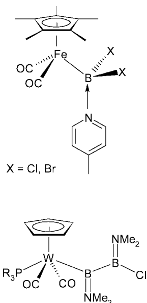
Figure 2. Methylpyridine Lewis base adduct of a \text{X}_2\text{B} -substituted iron complex and phosphane-substituted diborane(4)yl tungsten half-sandwich complex.
