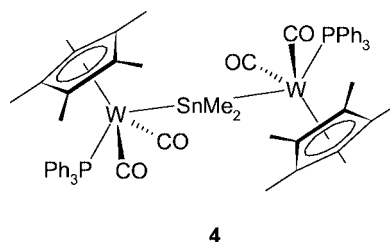
Figure 3. Disubstituted dimethylstannane trans - 4 .
