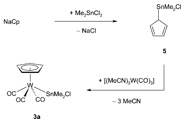
Scheme 1. Alternative synthesis of 3a via the chlorostannyl-functionalized cyclopentadiene 5 which is obtained from alkali salt elimination of sodium cyclopentadienyl and dichlorodimethyl stannane.
