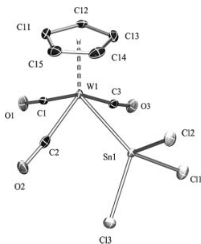
Figure 7. Molecular structure of [(\eta^5\text{-C}_5\text{H}_5)(\text{OC})_3\text{W}(\text{SnCl}_3)] ( 8 ) in the solid state with the atom-numbering scheme. Displacement ellipsoids are drawn at the 50% probability level and the hydrogen atoms have been omitted for clarity. Selected bond lengths [Å] and angles [°]: W1–C1 1.998(5), W1–C2 2.011(5), W1–C3 2.001(4), W1–Sn1 2.7244(3), Sn1–Cl1 2.3450(11), Sn1–Cl2 2.3616(11), Sn1–Cl3 2.3681(11), C1–W1–Sn1 126.42(12), C3–W1–Sn1 75.08(12), C2–W1–Sn1 76.17(12), Cl1–Sn1–Cl3 96.41(4), Cl1–Sn1–Cl2 98.94(4), Cl3–Sn1–Cl2 99.45(4), Cl1–Sn1–W1 121.81(3), Cl3–Sn1–W1 119.57(3), Cl2–Sn1–W1 116.14(3).
