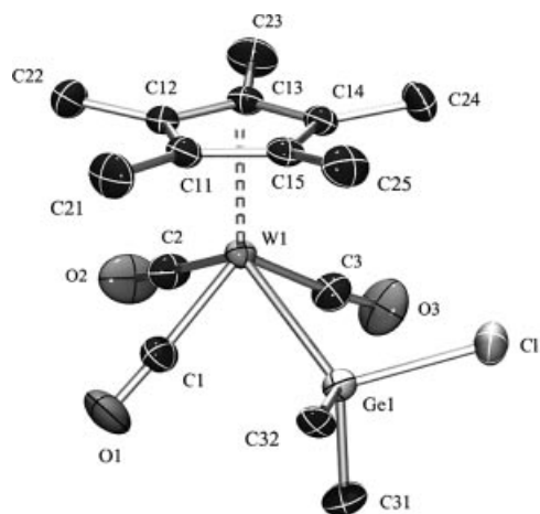
Figure 5. Molecular structure of [(\eta^5\text{-C}_5\text{Me}_5)(\text{OC})_3\text{W}(\text{GeMe}_2\text{Cl})] ( 3c ) in the solid state with the atom-numbering scheme. Displacement ellipsoids are drawn at the 50% probability level and the hydrogen atoms have been omitted for clarity. Selected bond lengths [Å] and angles [°]: W1–C1 1.971(4), W1–C2 1.982(4), W1–C3 1.982(4), W1–Ge1 2.6272(4), Ge1–C31 1.948(4), Ge1–C32 2.008(3), Ge1–Cl1 2.2428(10), C1–W1–Ge1 70.04(11), C2–W1–Ge1 123.98(11), C3–W1–Ge1 72.07(12), C31–Ge1–C32 106.44(17), C31–Ge1–Cl1 101.62(13), C32–Ge1–Cl1 101.97(10), C31–Ge1–W1 117.55(13), Cl1–Ge1–W1 109.74(3).
