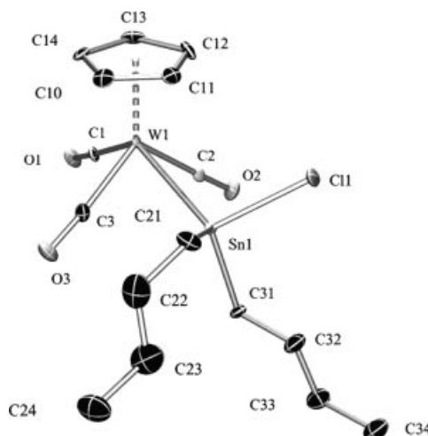
Figure 4. Molecular structure of [(\eta^5\text{-C}_5\text{H}_5)(\text{OC})_3\text{W}(\text{SnBu}_2\text{Cl})] ( 3b ) in the solid state with the atom-numbering scheme. Displacement ellipsoids are drawn at the 50% probability level and the hydrogen atoms have been omitted for clarity. Selected bond lengths [Å] and angles [°]: W1–C1 1.983(7), W1–C3 1.984(8), W1–C2 1.985(7), W1–Sn1 2.7959(5), Sn1–C31 2.156(7), Sn1–C21 2.168(8), Sn1–Cl1 2.4203(18), C31–Sn1–C21 114.6(3), C31–Sn1–Cl1 99.1(2), C21–Sn1–Cl1 99.6(2), C31–Sn1–W1 120.56(19), C21–Sn1–W1 114.1(2), Cl1–Sn1–W1 104.34(5).
